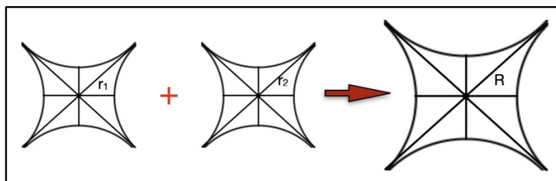
Figure 10a: Typical model of merger of 2 numbers of 2D saddles to form a larger 2D saddle
