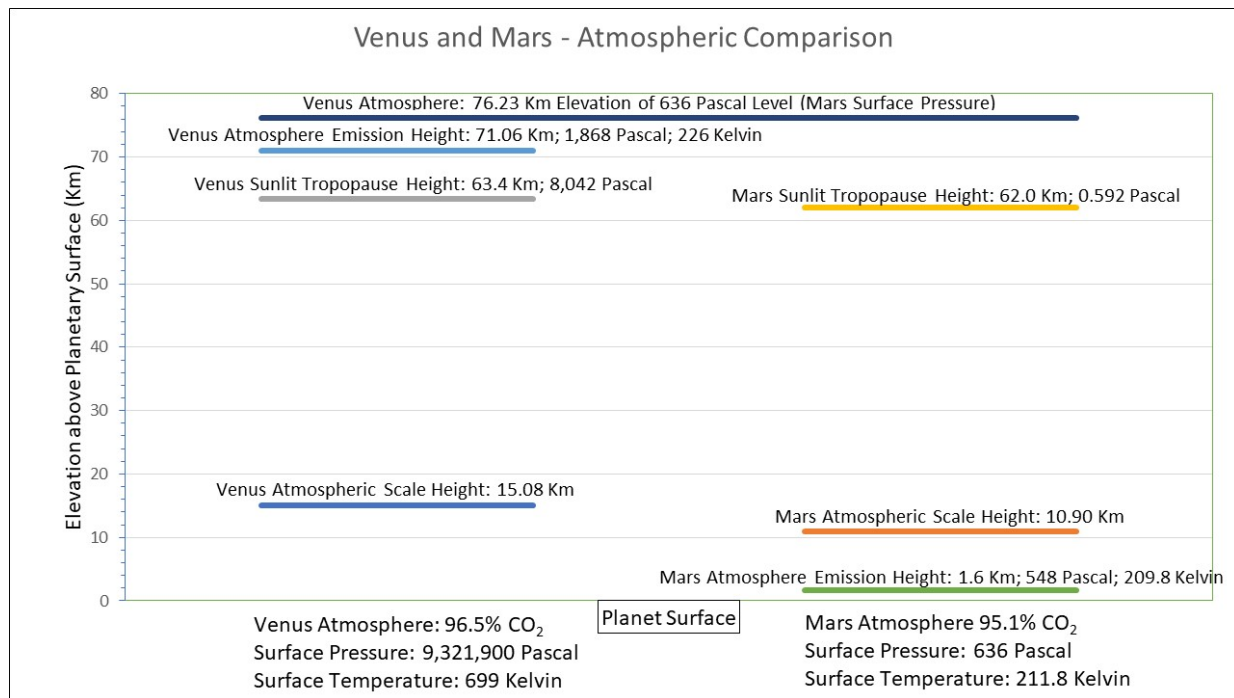
Figure 3: Venus and Mars - Atmospheric Comparison
