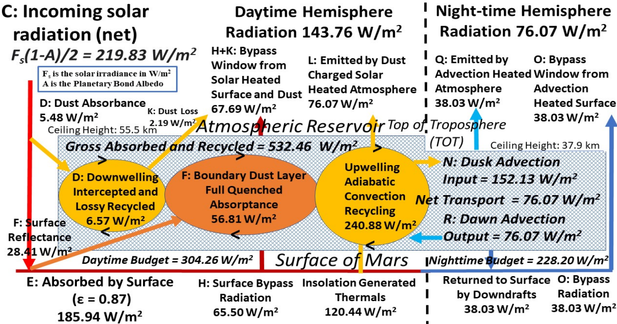
Figure 5: The Atmospheric Energy Flux Reservoir of Dust Opaque Mars Generated by the Adiabatic Convection Recycling of Surface Thermal Conduction Energy
