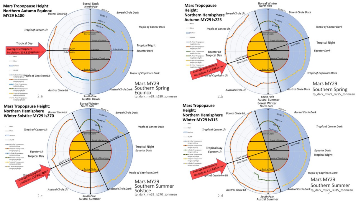
Figure 2: Mars Global Tropopause Height - Southern Hemisphere Summer
